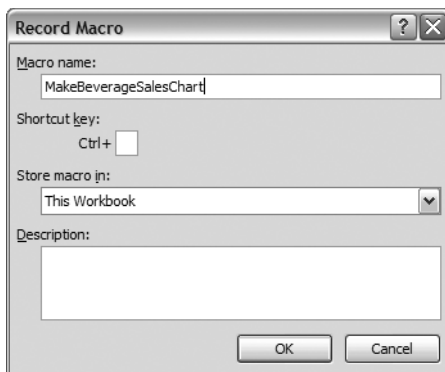
Figure 5-2. Recording the MakeBeverageSalesChart macro
