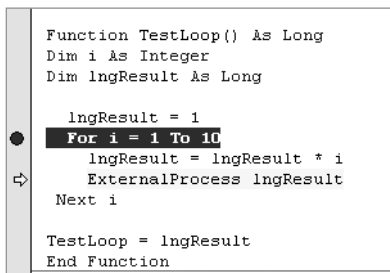
Figure 7-23. The Set Next Statement command moves the execution point to the selected line of code.
