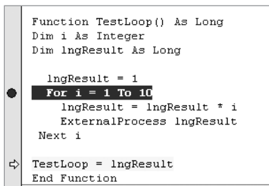
Figure 7-24. The Run To Cursor command moves the execution point to the cursor location.
