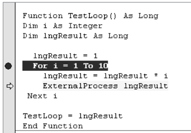
Figure 7-21. Execution point on a procedure call
