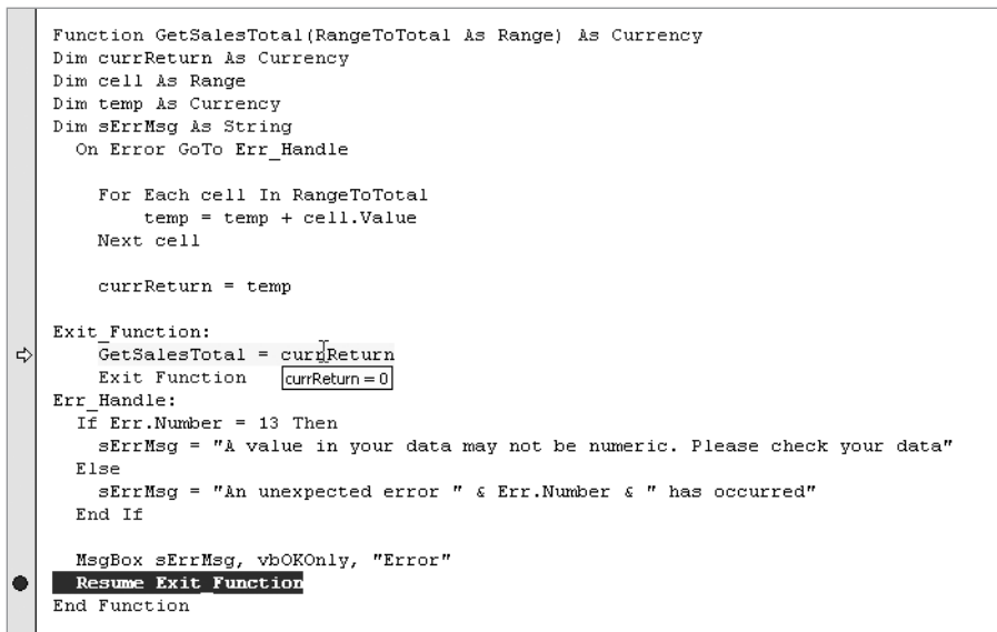
Figure 7-44. Checking the value of currReturn
