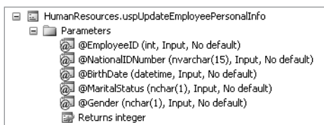
Figure 2-28. uspUpdateEmployeePersonalInfo and parameters
