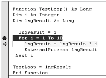
Figure 7-19. Better view of the break and execution lines of code
