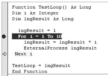
Figure 7-22. The execution point moves directly to the next line of code when the Step Over command is used.
