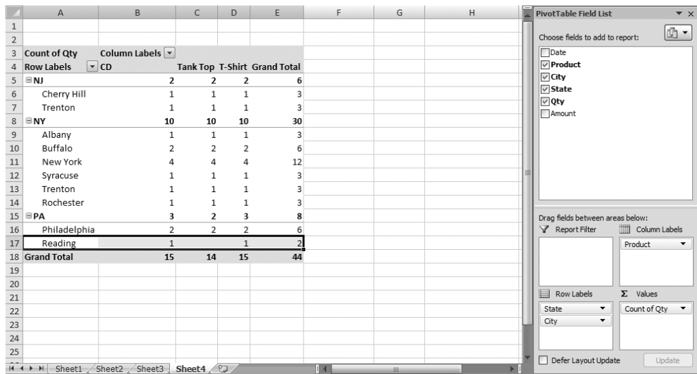
Figure 6-17. Count of Qty is the default due to the blank data record.
